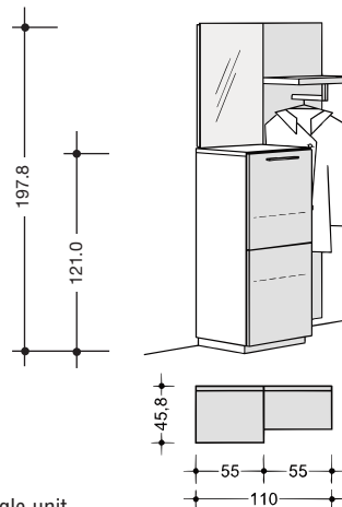
6 Raster single unit with door hinge left
