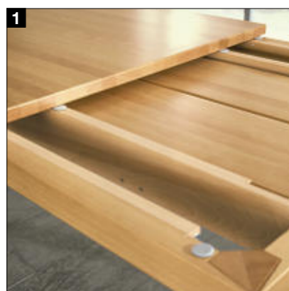
ET 800 Table top: solid wood/5-layer solid wood board Leg versions: solid wood Versions: solid wood: solid alder; 5-layer solid wood board: solid beech, solid natural oak Table lengths: 160, 180 and 200 cm Extendable: 160-220/280 cm, 180-240/300 cm and 200-260/320 cm
